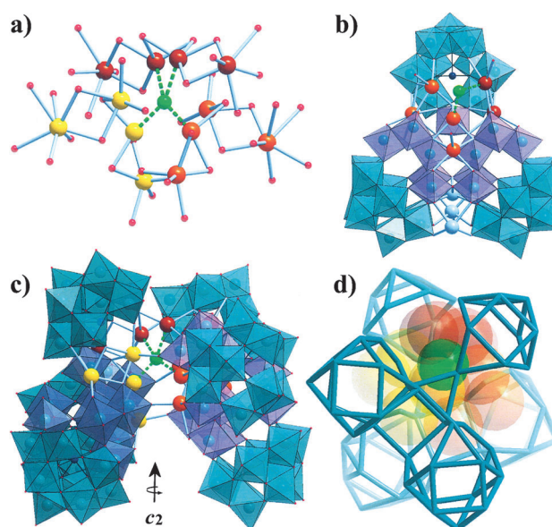
Figure 1. Structural aspects of 1 . a) {Ag 12 Cl} core with the four direct Ag–Cl bonding interactions shown. The three non-interacting groups of Ag cations are also highlighted. b) {Te 3 W 38 } half unit found in 1–3 with the coordinated Ag + cations shown. c) The fully assembled structural unit of 1 . d) A pictographic representation of 1 highlighting the twisted orientation of the two {Te 3 W 38 } half units with respect to another around the central {Ag 12 Cl} core. Cations and water molecules are omitted. ({TeW 9 } units are shown as teal/aqua polyhedra, {W 11 } units are shown in lavender/blue gray polyhedra. O: red, Te: dark blue, Ag: brown, orange, and gold, Cl: green).
